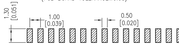
Recommended P.C.B Layout(Top Side) (PCB BOARD TOLERANCE±0.05)
