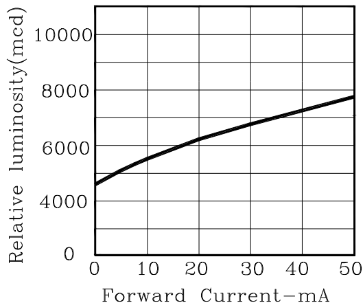
Forward Current vs. Relative luminosity
