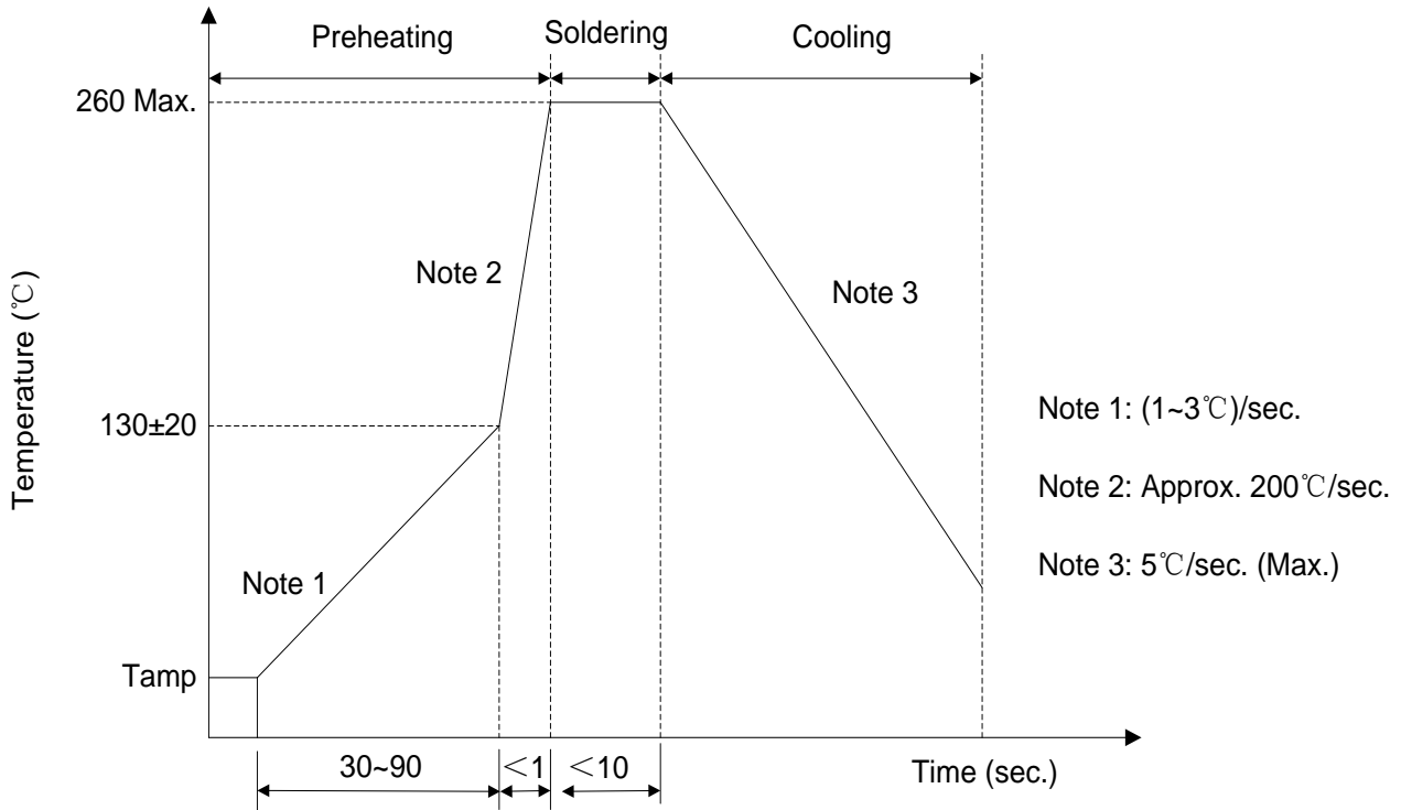
Wave Soldering Recommendation
